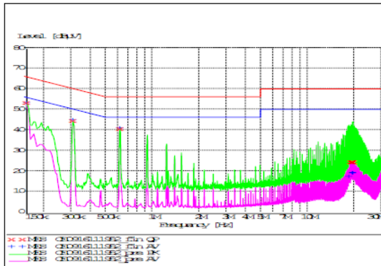
Figure 24. EMC Considerations.
