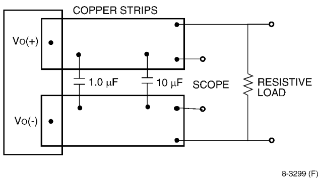
Figure 13. Output Ripple and Noise Test Setup.
