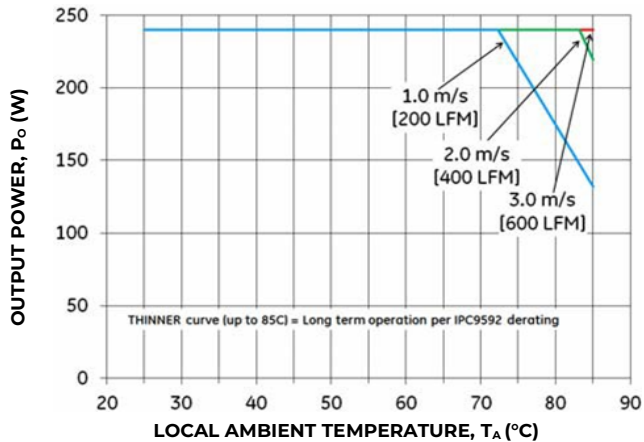
Figure 17. Output Power Derating for the Open Frame EBVE025A0S9R6 in the Transverse Orientation; Airflow Direction from V_{in(-)} to V_{in(+)} ; V_{in} = 55V .
