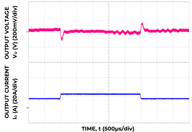
Figure 4. Typical Transient Response to 1A/ \mu s Step Change in Load from 50% to 75% to 50% of Full Load, C_o = 1200\mu F and 50 V dc Input.
