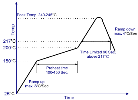
Figure 21. Recommended linear reflow profile using Sn/Ag/Cu solder.
