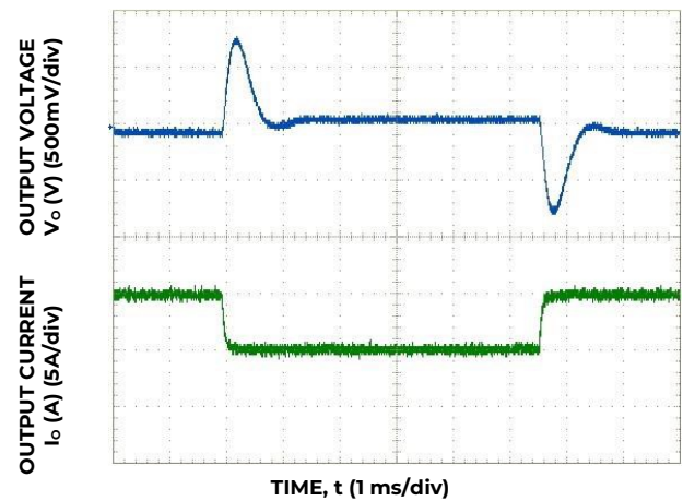
Figure 6. Typical Transient Response to Step Change in Load from 50% to 75% to 50% of Full Load at 48Vdc Input and C_O = 470\mu F Polymer, without -02 option.
