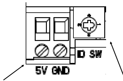
5V termination - Shelf ID switch for I 2 C addressing(1 - 4)
