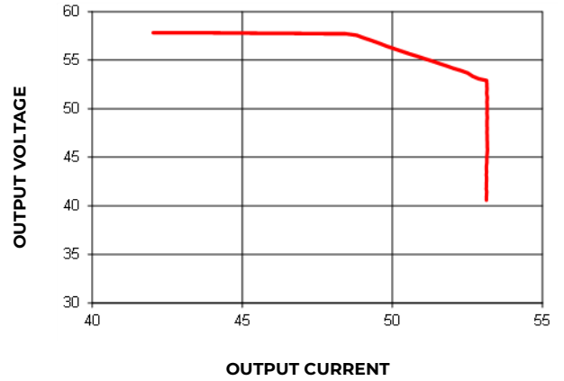
Figure 2. 56V DC output: Power limit, Current limit and shutdown profile at V_{IN} = 185V_{AC}
