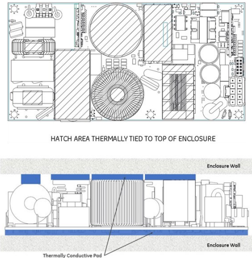
Fig. 1. Example arrangement of the CLP0612 for sealed enclosure applications.
