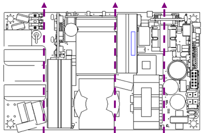
Fig 2. Preferred airflow direction for cooling.
