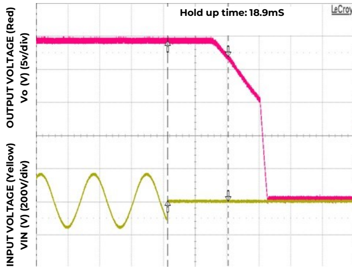
Figure 6. Typical Hold-up Waveforms (VIN = 115Vac, 100% Load)
