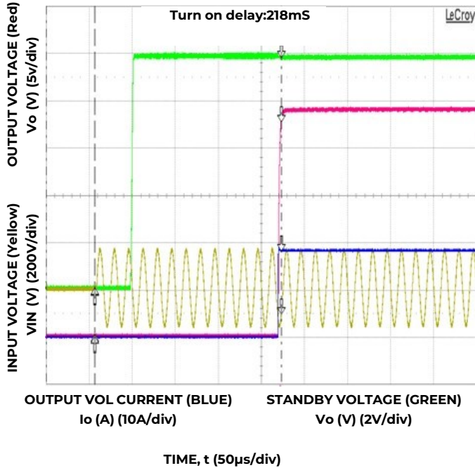
Figure 4. Typical Start-up (VIN = 115Vac, Full Load)
