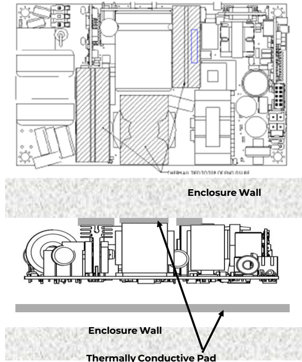
Fig 1. Example arrangement of the CLP0424/28 for sealed enclosure applications.
