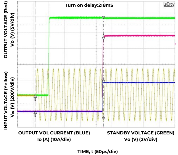
Figure 5. Typical Start-up (VIN = 230V, Full Load)
