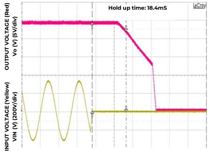
Figure 7. Typical Hold-up Waveforms (VIN = 230V, 100% Load)
