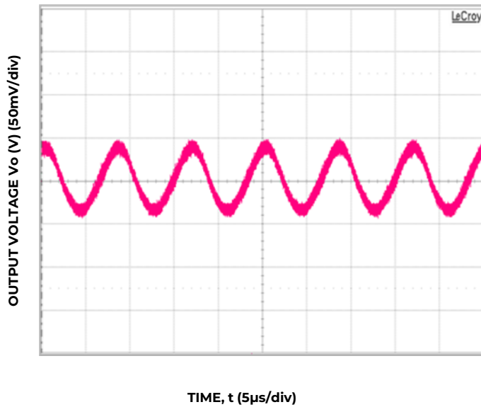
Figure 2. Typical output ripple and noise (VIN = 230Vac, 100% load )
