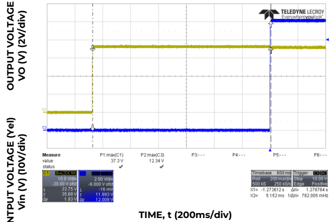
Figure 4. Minimum Input Start-up ( V_{IN} = 36V_{dc} , Full Load).
