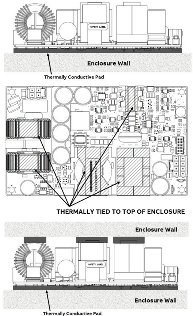
Fig. 11. Example arrangement of the CLP0412DC for sealed enclosure applications
