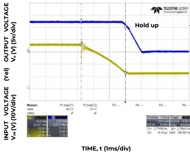
Figure 6. Minimum input Hold-up waveforms ( V_{IN} = 36V , 100% Load).
