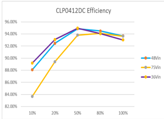
Figure 1: Power Supply Efficiency Versus Output Current
