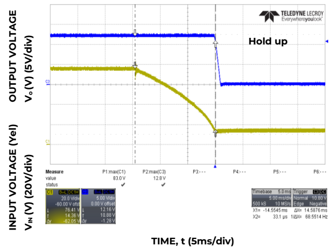
Figure 7. Maximum input Hold-up waveforms ( V_{IN} = 75V , 100% Load).
