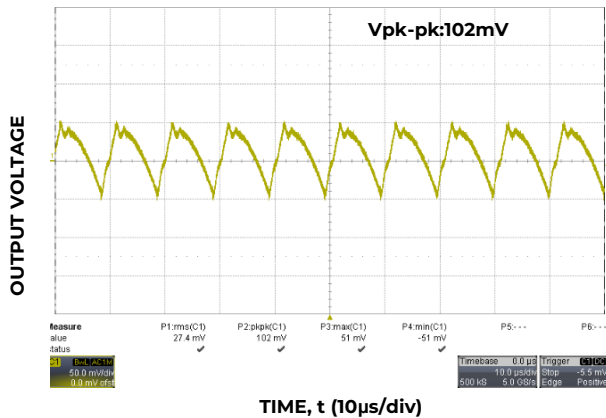
Figure 2. Typical output ripple and noise ( V_{IN} = 48V_{dc} , 100% load)
