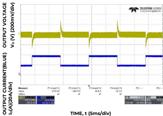
Figure 3. Transient Response to Dynamic Load Change from 50% to 100% at V_{IN} = 48V_{dc}
