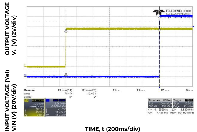
Figure 5. Maximum Input Start-up ( V_{IN} = 75V_{dc} , Full load).
