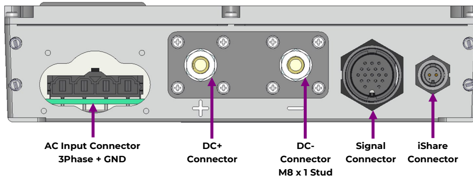
Connectors without mated pairs, covers and cables
