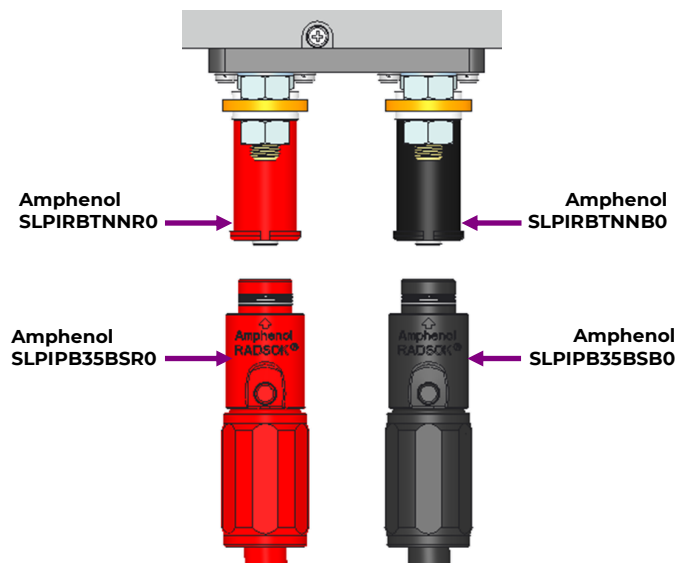
Rectifier output connectors with busbar kit assembled (cables not included)
