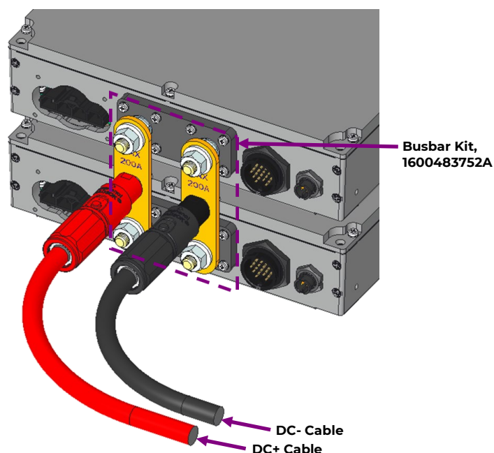
Connectors with mated pairs, covers, cables, busbar kit
