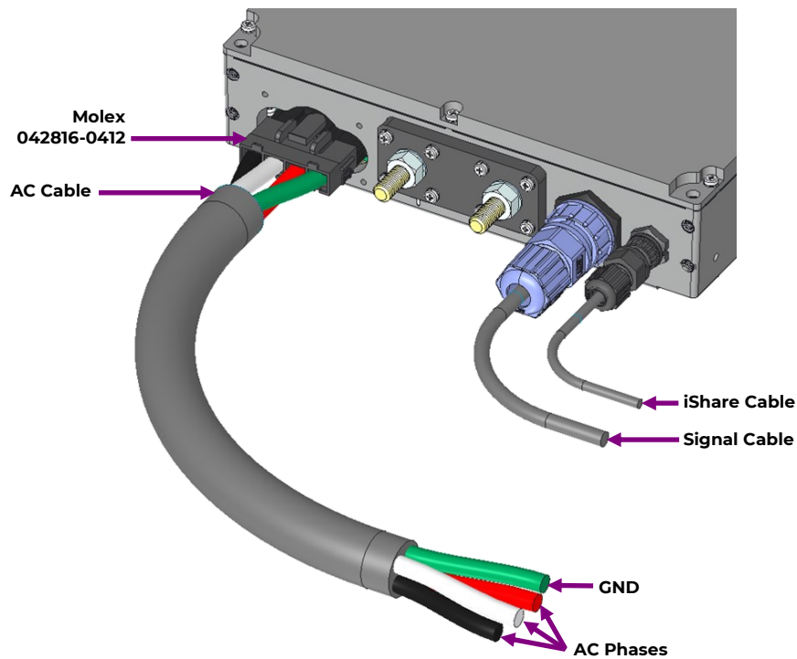
Connectors with mated pairs, covers and cables
