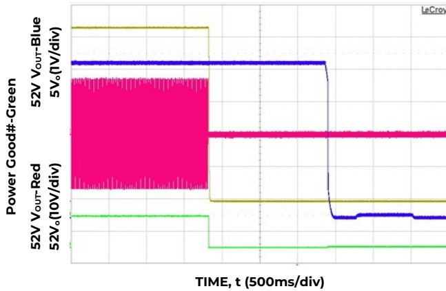
Figure 15. Turn-OFF at full load, V_{IN}=230V_{AC}
