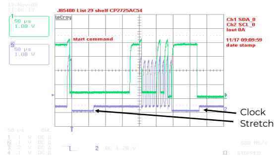
Figure 15. Example waveforms showing clock stretching.
