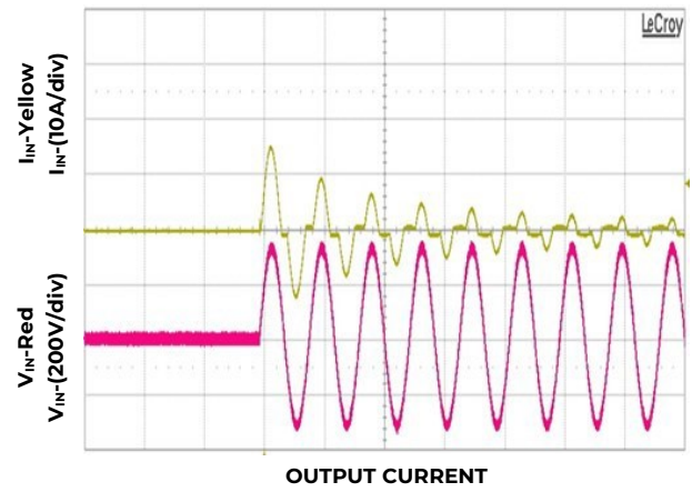
Figure 2. Inrush current V IN = 230V AC , 0°C phase angle
