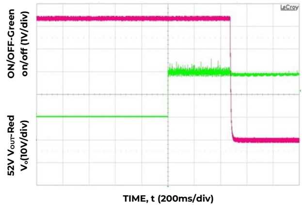
Figure 16. 52V DC turn-OFF delay when ON/OFF is dis- serted, V_{IN}=230V_{AC} - I 2 C mode.
