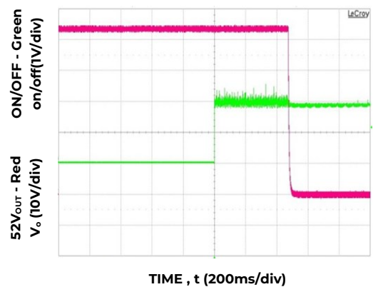
Figure 16. 52V DC turn-OFF delay when ON/OFF is di-asserted, V_{IN}=230V_{AC} - I 2 C mode
