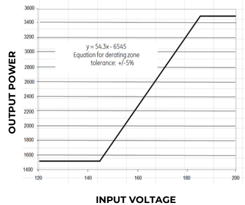
Figure 18. Output power derating below V_{IN} of 185V AC
