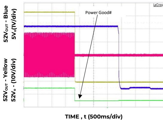
Figure 15. Turn-OFF at full load, V_{IN}=230V_{AC}
