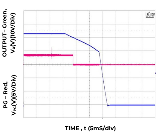
Figure 12. PG# alarmed 10ms prior to V o < 40V, V IN = 230V AC , Output at Full load
