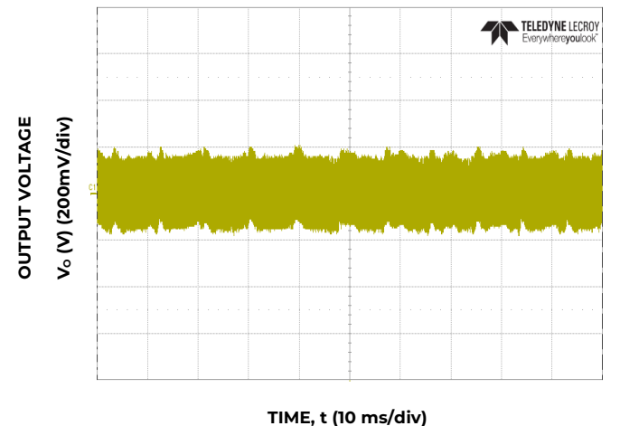
Figure 6. 8 V_{DC} output ripple and noise, all full load, V_{IN} = 230V_{AC} , 20 MHz bandwidth
