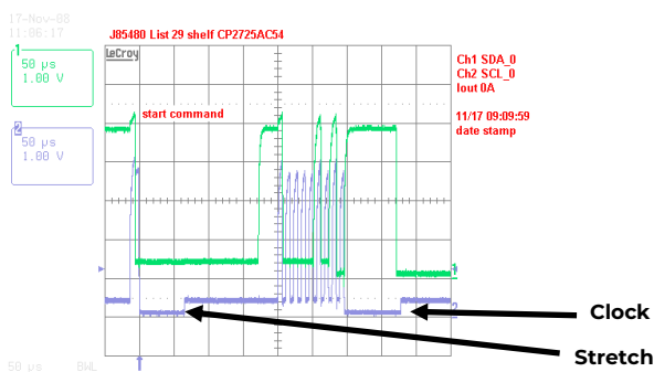
Figure 1. Example waveforms showing clock stretch
