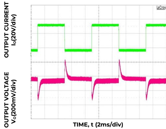
Figure 7. 12V transient response for 10 to 60% step load, V_{in} : - 48V DC , slew rate 1A/ \mu s
