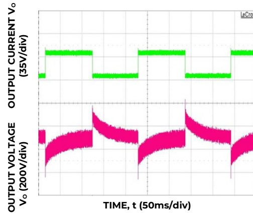
Figure 8. 12V transient response for 50 to 100% step load, V_{in} : - 48V DC , slew rate 1A/ \mu s.
