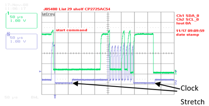
Figure 14. Example waveforms showing clock stretching.
