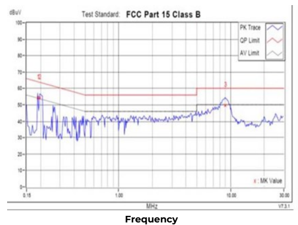
Figure 12. Conducted Emissions
