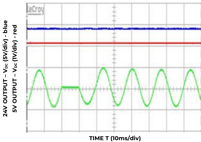
Figure 8. \frac{1}{2} cycle ride-through V_{IN} 140 V_{AC}
