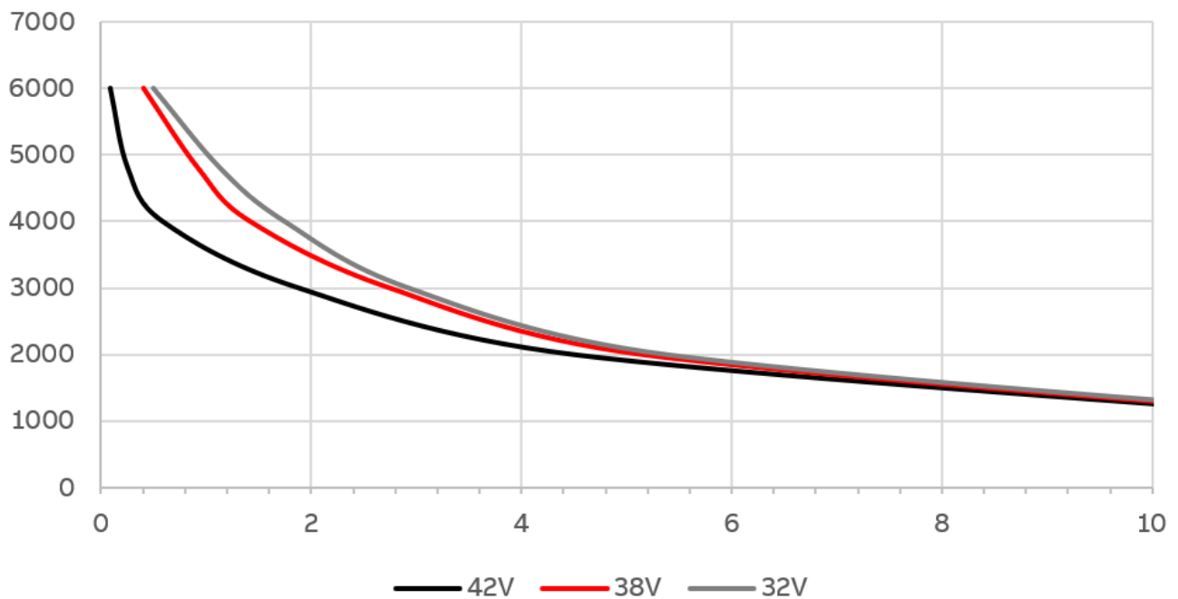
Output to end cell voltage @25°C (Watts/Minutes)
