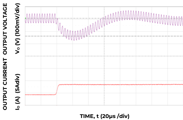
Figure 17. Transient Response to Dynamic Load Change from 50% to 100% at 28V in , C ext = 1x22µF+1x470µF, C Tune =1.5nF & R Tune =200
