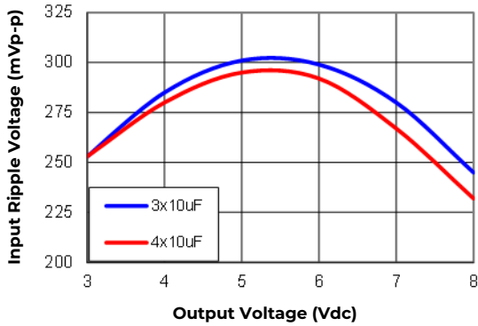
Figure 30. Input ripple voltage for various output voltages with 3x10 \mu F or 4x10 \mu F ceramic capacitors at the input (maximum load). Input voltage is 12V. Scope BW at 20MHz
