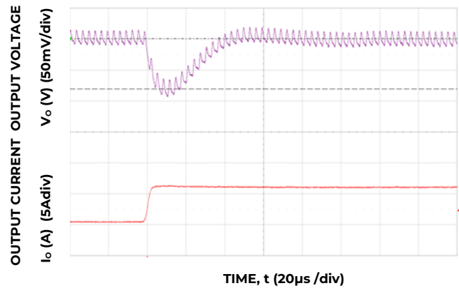
Figure 10. Transient Response to Dynamic Load Change from 50% to 100% at 28Vin, C ext – 1X22µF+1x330µF, C Tune =5.6nF & R Tune =200.
