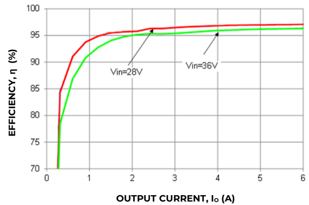
Figure 22. Converter Efficiency versus Output Current. (-78 Version)
