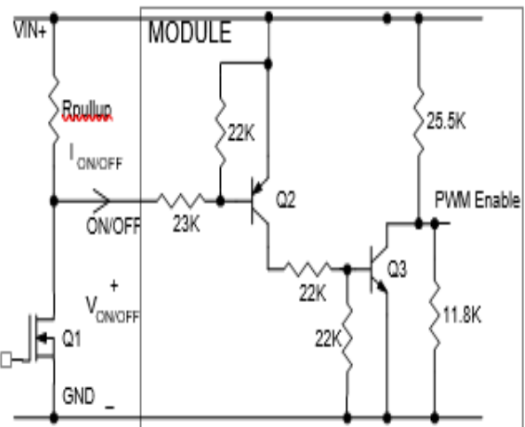
Figure 42. Circuit configuration for using positive On/Off logic.
