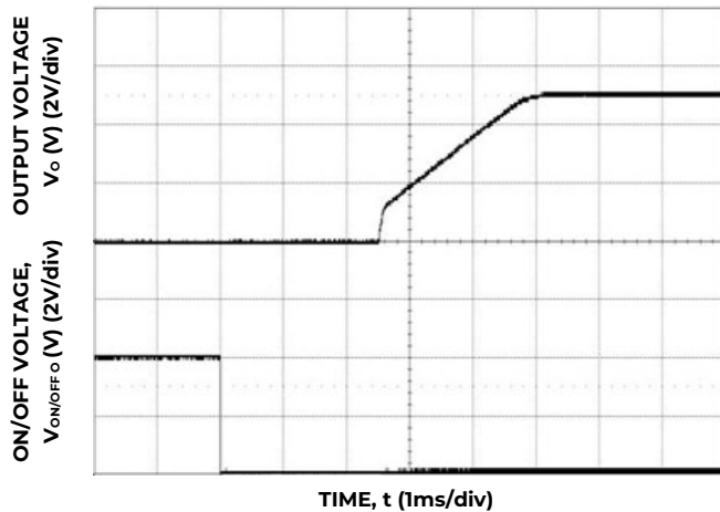
Figure 33. Typical Start-up Using On/Off Voltage ( I_o = I_{o,max} ).
