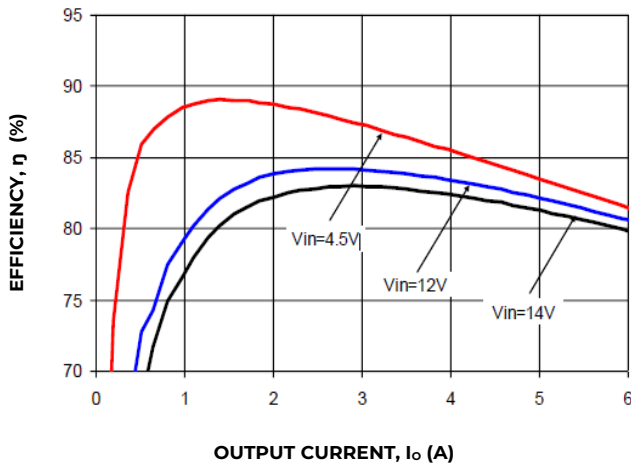
Figure 7. Converter Efficiency versus Output Current.
