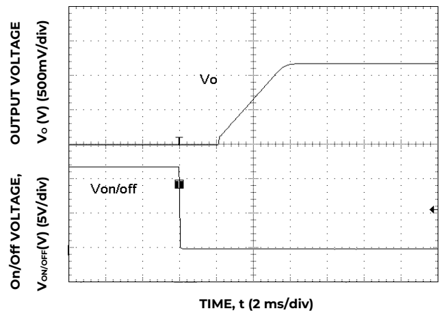
Figure 11. Typical Start-up Using On/Off Voltage ( I_o = I_{o, \text{max.}} ).
