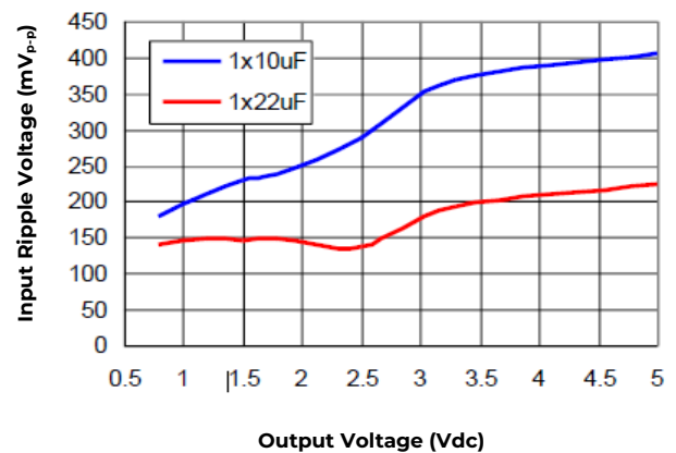
Figure 40. Input ripple voltage for various output voltages with 1x10\mu F or 1x22\mu F ceramic capacitors at the input (6A load). Input voltage is 12V.
