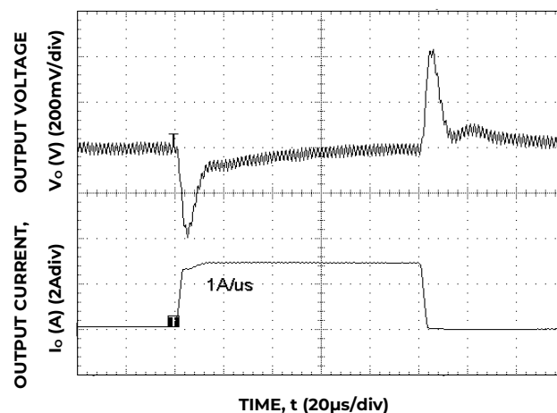
Figure 28. Transient Response to Dynamic Load Change from 50% to 0% .
