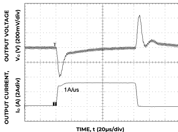
Figure 22. Transient Response to Dynamic Load Change from 50% to 0% .
