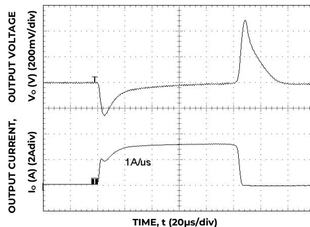
Figure 4. Transient Response to Dynamic Load Change from 50% to 0% .
