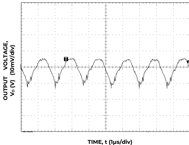
Figure 9. Typical Output Ripple and Noise, V_{IN} = 12 \text{ V} I_o = I_{o, \text{max.}}
