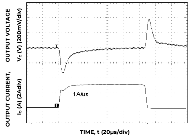
Figure 10. Transient Response to Dynamic Load Change from 50% to 0% .
