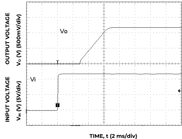
Figure 12. Typical Start-up Using Input Voltage ( V_{IN} = 12 \text{ V} I_o = I_{o, \text{max.}} )
