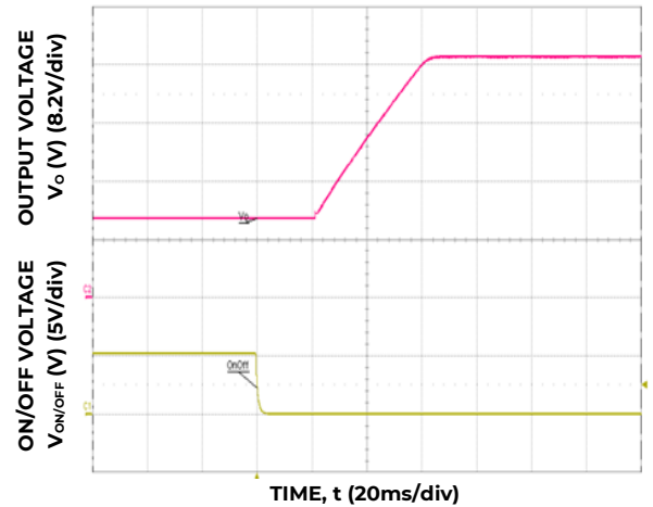
Figure 23. Typical Start-up Using On/Off Voltage ( I_o = I_{o,max} ).
