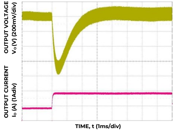
Figure 22. Transient Response to Dynamic Load Change from 0.9A to 1.9A at 12V in , C out =470uF, C Tune =1000pF, R Tune =30.1kΩ
