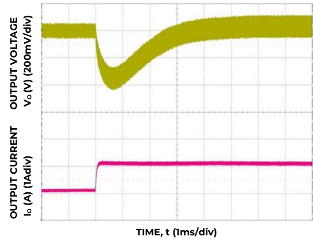
Figure 16. Transient Response to Dynamic Load Change from 50% to 100% at 12V in , C out =470uF, C Tune =1000pF, R Tune =30.1kΩ
