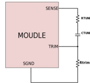
Figure 30. Circuit diagram showing connection of R_{TUNE} and C_{TUNE} to tune the control loop of the module
