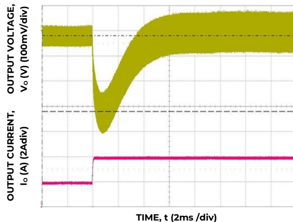
Figure 4. Transient Response to Dynamic Load Change from 50% to 100% at 12V in , C_{out}=3x10uF+470uF , C_{Tune}=1000pF , R_{Tune}=30.1k\Omega
