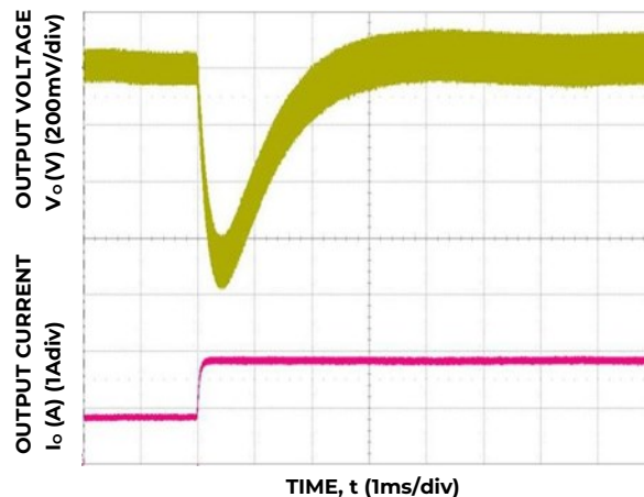
Figure 22. Transient Response to Dynamic Load Change from 0.9A to 1.9A at 12V in , C_{out} = 470 \mu F , C_{Tune} = 1000 pF , R_{Tune} = 30.1 k\Omega
