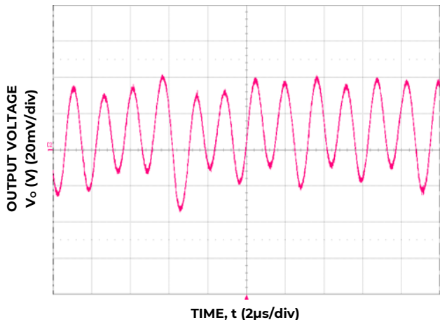
Figure 9. Typical output ripple and noise ( C_o=3 \times 10 \mu F + 470 \mu F , V_{IN} = 12V , I_o = I_{o,max} ).
