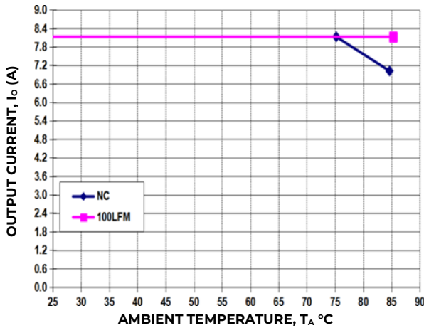
Figure 2. Derating Output Current versus Ambient Temperature and Airflow., V IN =12V
