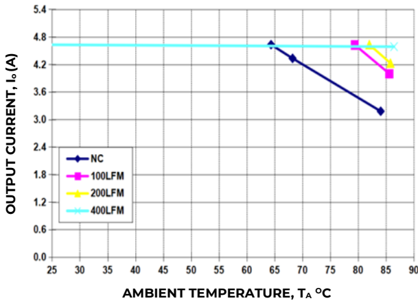
Figure 14. Derating Output Current versus Ambient Temperature and Airflow. V_{IN} = 12V
