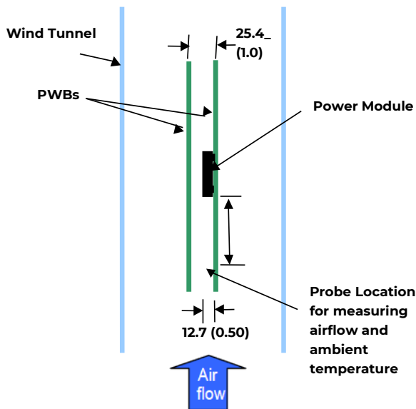
Figure 31. Thermal Test Setup.
