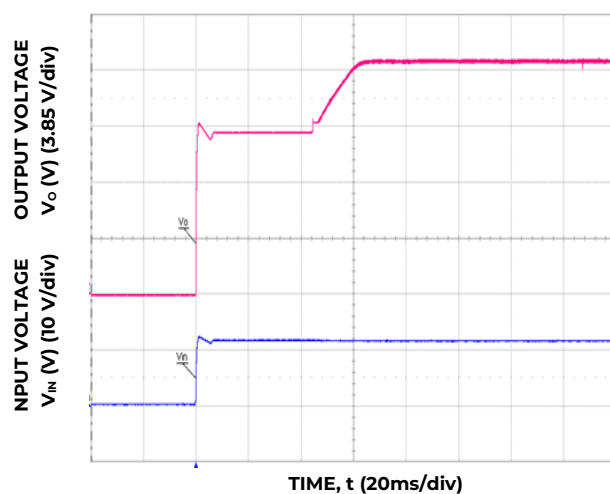
Figure 6. Typical Start-up Using Input Voltage ( V_{IN} = 12V , I_o = I_{o,max} ).
