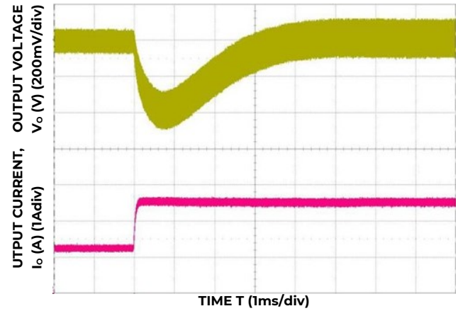
Figure 10. Transient Response to Dynamic Load Change from 50% to 100% at 12 V_{in} , C_{out}=3 \times 10 \mu F + 470 \mu F , C_{Tune}=1000 pF , R_{Tune}=30.1 k\Omega
