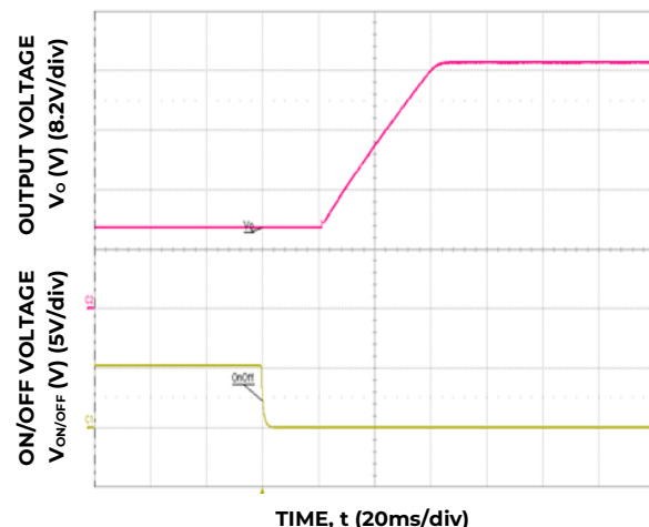
Figure 23. Typical Start-up Using On/Off Voltage ( I_o = I_{o,max} ).
