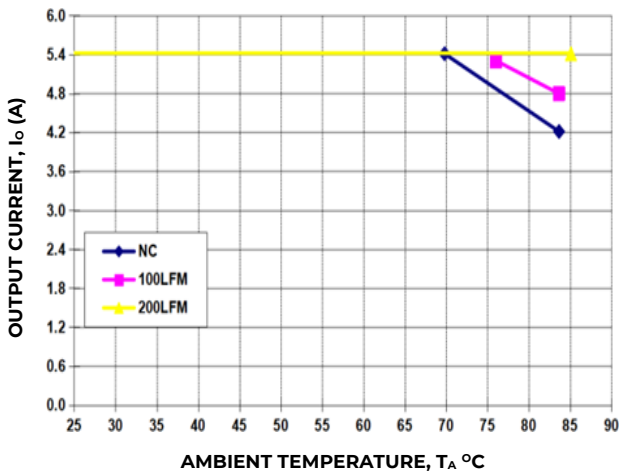
Figure 8. Derating Output Current versus Ambient Temperature and Airflow, V_{IN}=12V
