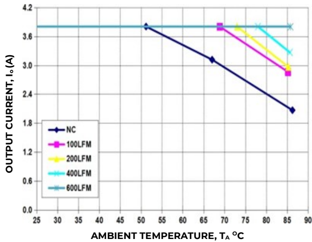
Figure 20. Derating Output Current versus Ambient Temperature and Airflow. V_{IN} = 12V
