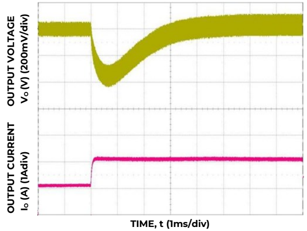
Figure 16. Transient Response to Dynamic Load Change from 50% to 100% at 12V in , C out =470uF, C Tune =1000pF, R Tune =30.1kΩ
