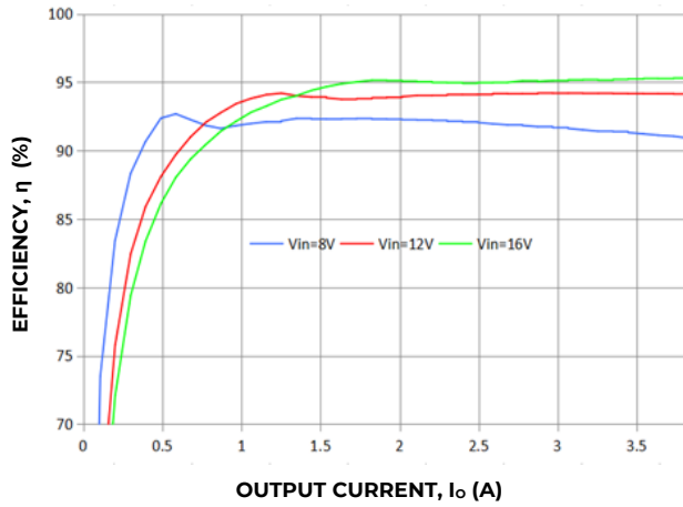
Figure 19. Converter Efficiency versus Output Current.
