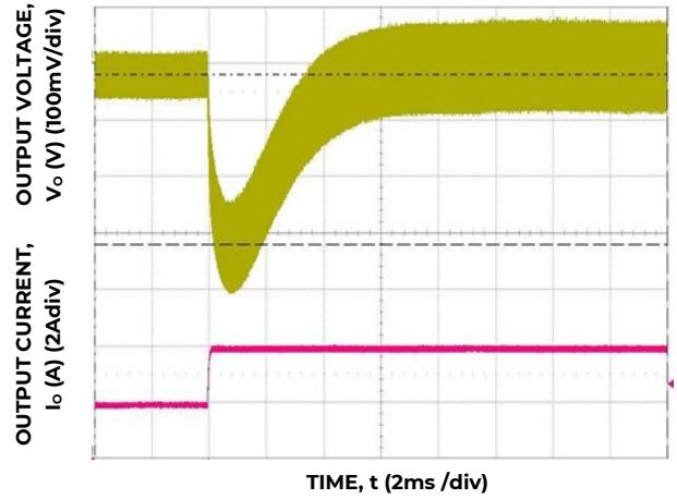
Figure 4. Transient Response to Dynamic Load Change from 50% to 100% at 12V in , C out =3x10uF+470uF, C Tune =1000pF, R Tune =30.1kΩ
