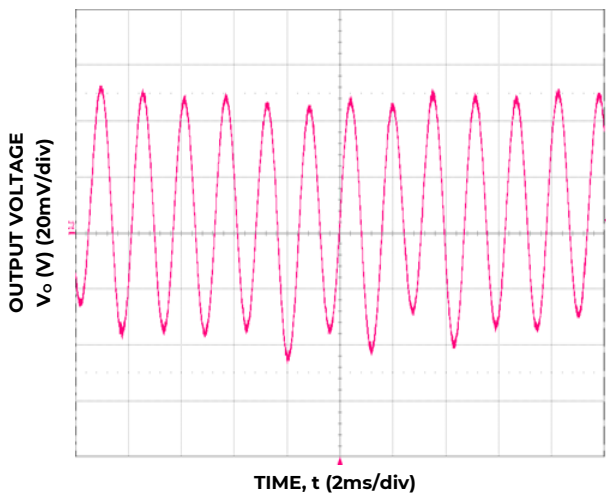
Figure 3. Typical output ripple and noise (C o =3x10uF+470uF, V IN = 12V, I o = I o,max ).
