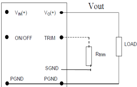
Figure 28. Circuit configuration for programming output voltage using an external resistor.
