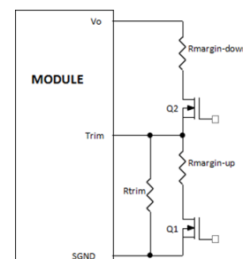
Figure 29. Circuit Configuration for margining Output voltage.
