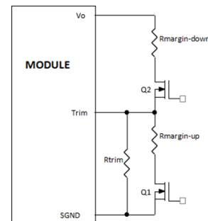
Figure 29. Circuit Configuration for margining Output voltage.
