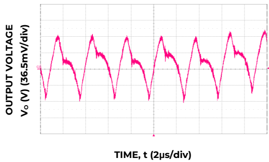
Figure 3. Typical output ripple and noise ( C_o=3x10uF+470uF , V_{IN} = 12V , I_o = I_{o,max} ).
