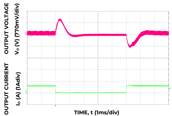
Figure 22. Transient Response to Dynamic Load Change from 50% to 0% at 12V in , C_{out}=470uF , C_{Tune}=1000pF , R_{Tune}=30.1k\Omega
