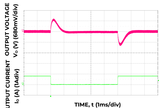
Figure 16. Transient Response to Dynamic Load Change from 50% to 0% at 12V_{in} , C_{out}=470 \mu F , C_{Tune}=1000pF , R_{Tune}=30.1k\Omega
