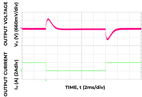
Figure 4. Transient Response to Dynamic Load Change from 50% to 0% at 12V in , C_{out}=3x10uF+470uF , C_{Tune}=1000pF , R_{Tune}=30.1k\Omega
