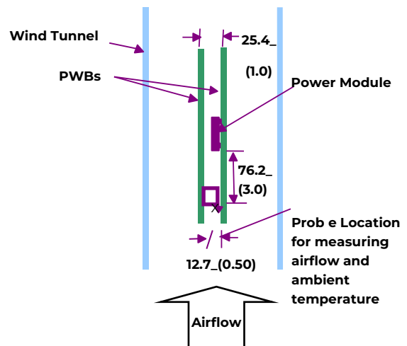
Figure 32. Thermal Test Setup
