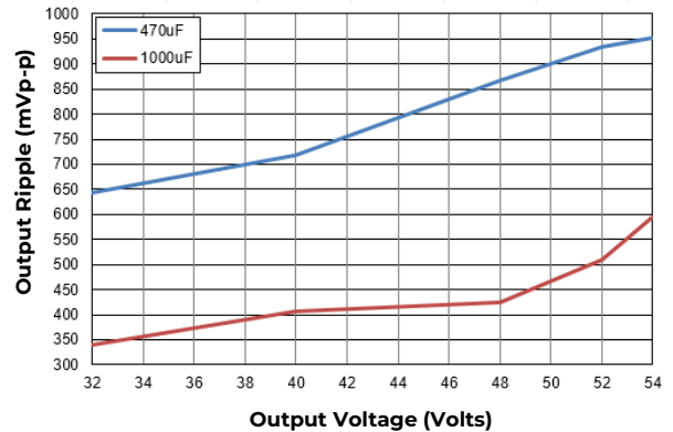
Figure 26. Output ripple voltage. Input voltage is 12V. Scope BW Limited to 20MHz
