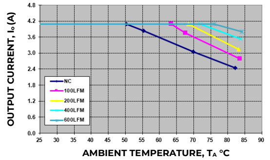
Figure 8. Derating Output Current versus Ambient Temperature and Airflow., V_{IN}=12V
