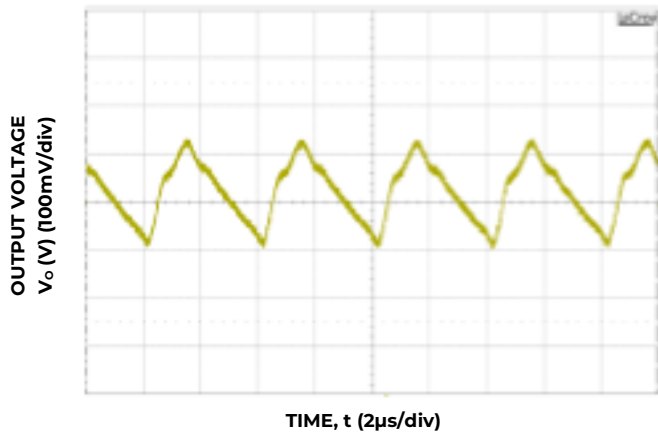
Figure 3. Typical output ripple (C o =66µF ceramic, V IN = 12V, I o = I o,max ).
