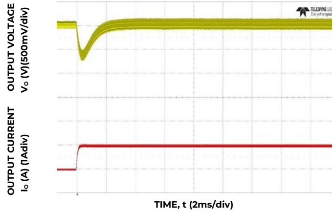
Figure 4. Transient Response to Dynamic Load Change from 50% to 100% at 12V in , C out = 12x4.7µF, C Tune =820pF, R Tune =30.1Ω
