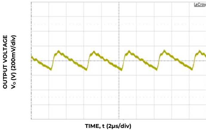
Figure 21. Typical output ripple and noise (C o =66μF ceramic, V IN = 12V, I o = I o,max ).
