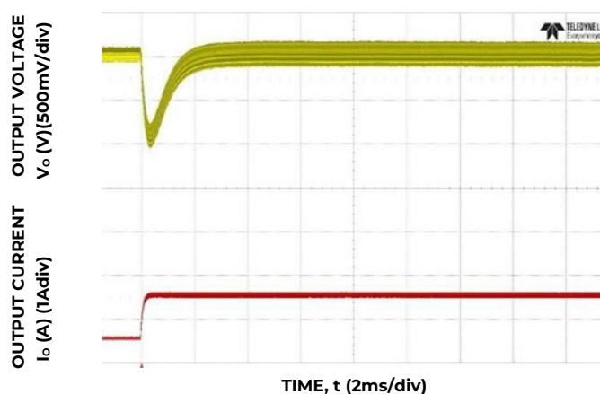
Figure 10. Transient Response to Dynamic Load Change from 0.6 to 1.6A at 12Vin, C out =10x4.7µF, C Tune =560pF, R Tune =40.2k
