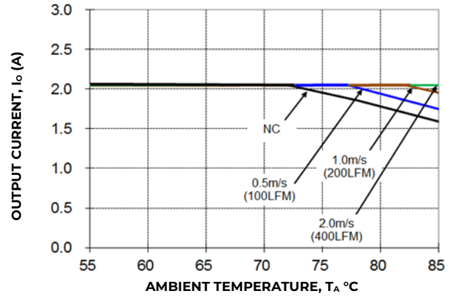
Figure 2. Derating Output Current versus Ambient Temperature and Airflow. Vin = 12V
