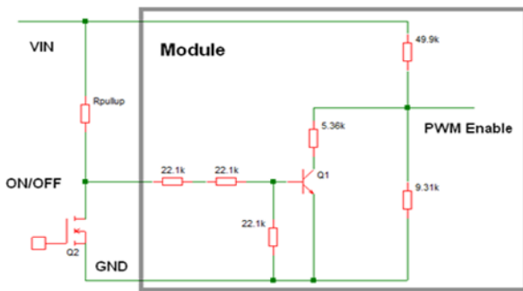
Figure 28. Circuit configuration for using negative On/Off logic.
