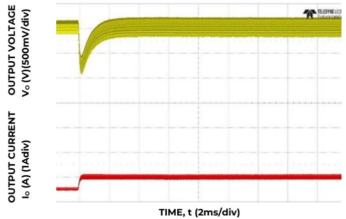
Figure 22. Transient Response to Dynamic Load Change from 0.6 to 1.1A at 12V in , C out = 7x4.7μF C tune =82pF, R tune =40.2Ω
