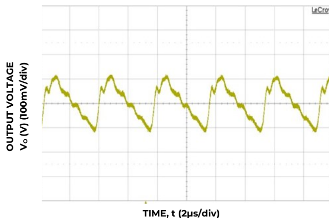
Figure 9. Typical output ripple and noise (C o =66µF ceramic, V IN = 12V, I o = I o,max ).
