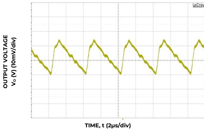
Figure 15. Typical output ripple and noise (C o =66μF ceramic, V IN = 12V, I o = I o,max ).
