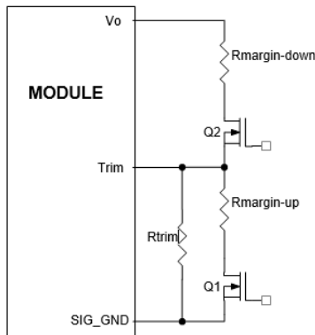
Figure 31. Circuit Configuration for margining Output voltage.
