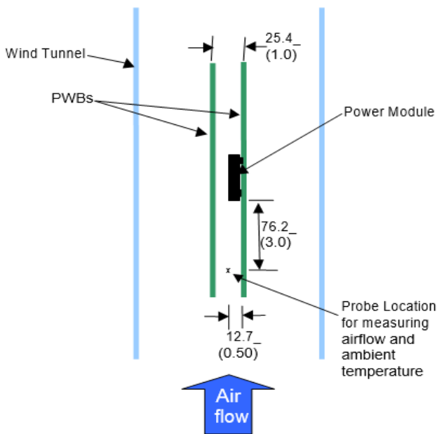
Figure 33. Thermal Test Setup.
