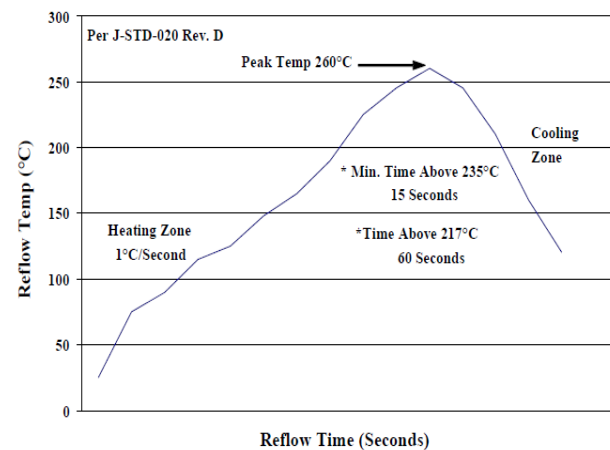
Figure 35. Recommended linear reflow profile using Sn/Ag/Cu solder.
