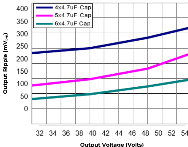
Figure 27. Output ripple voltage. input voltage is 12V. Scope BW Limited to 20MHz
