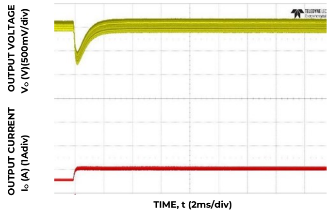
Figure 16. Transient Response to Dynamic Load Change from 0.65A to 1.15A at 12V in , C out =9x4.7uF, C Tune =220pF, R Tune =40.2kΩ
