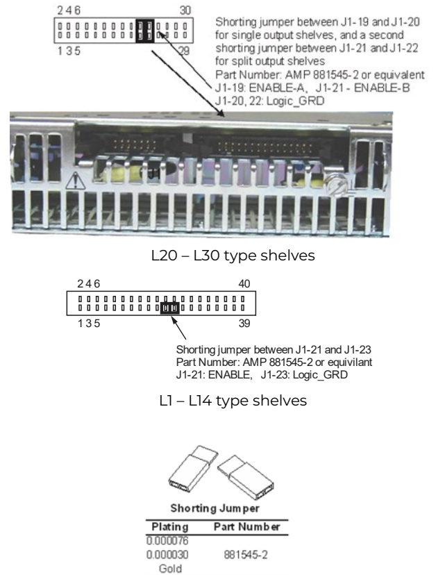
Jumper positioned into the J1 signal connector
