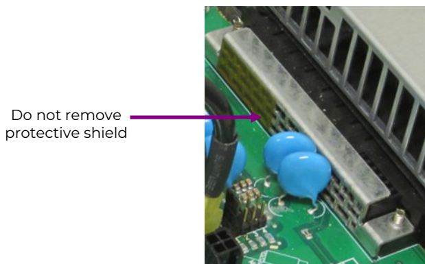
Figure 7 - Protective Shield
