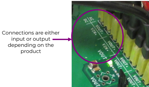
Figure 6 - Power Connections
