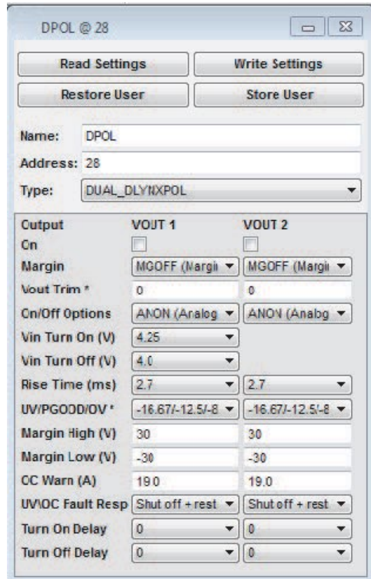
Figure 4. ProGUI Dual Output POL Parameter Window.
